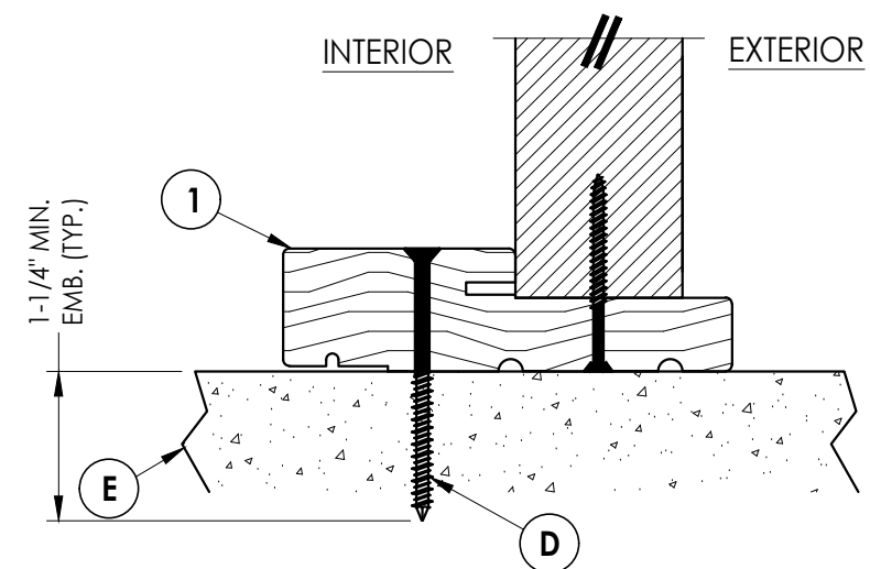
7 3 VERTICAL CROSS SECTION Outswing Sill
